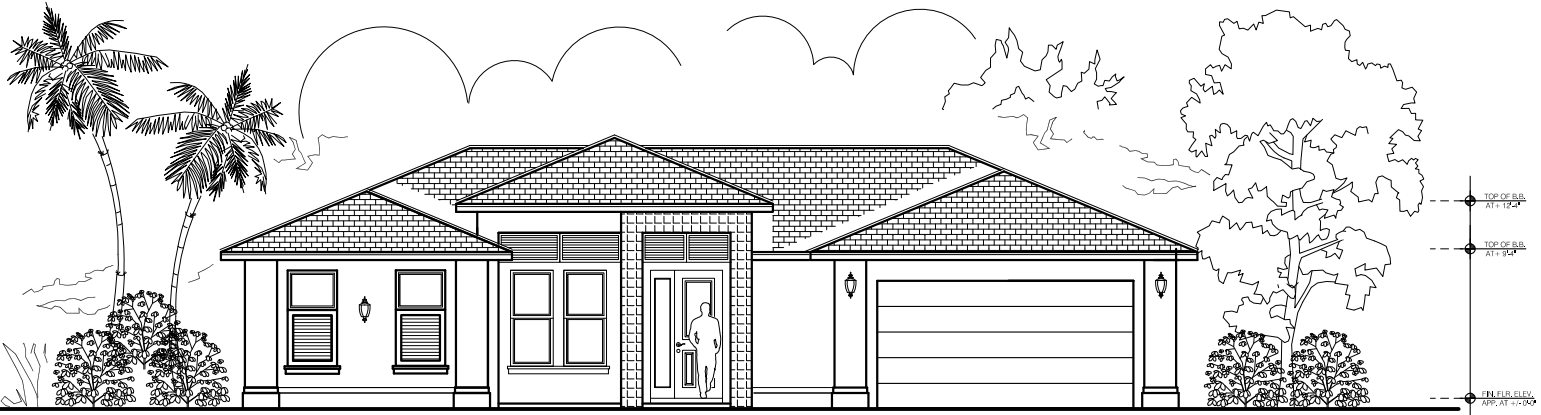
RESIDENCE FRONT ELEVATION
