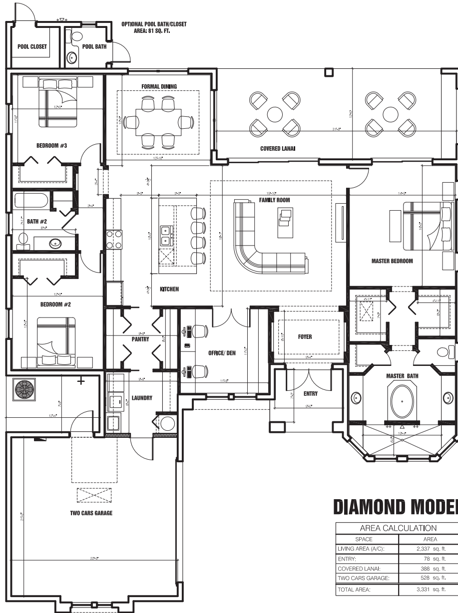
RESIDENCE FLOOR PLAN
