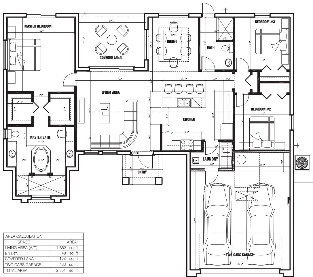
RESIDENCE FLOOR PLAN
