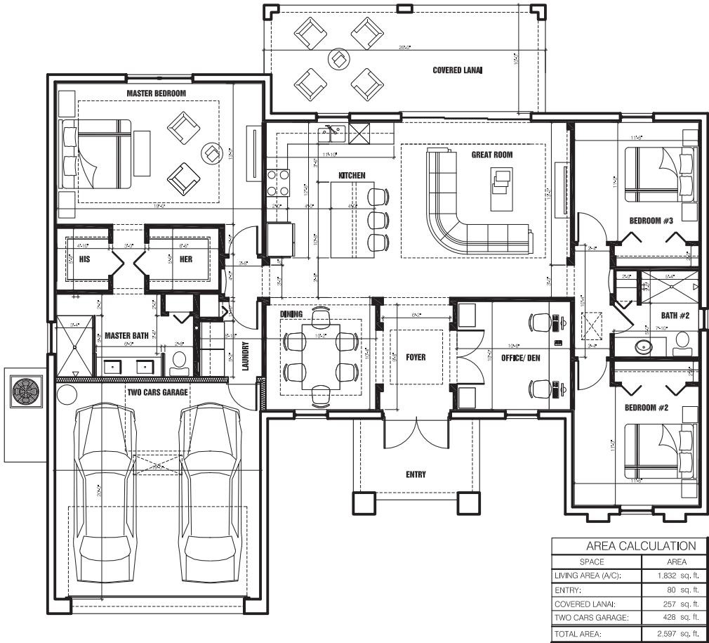
RESIDENCE FLOOR PLAN
